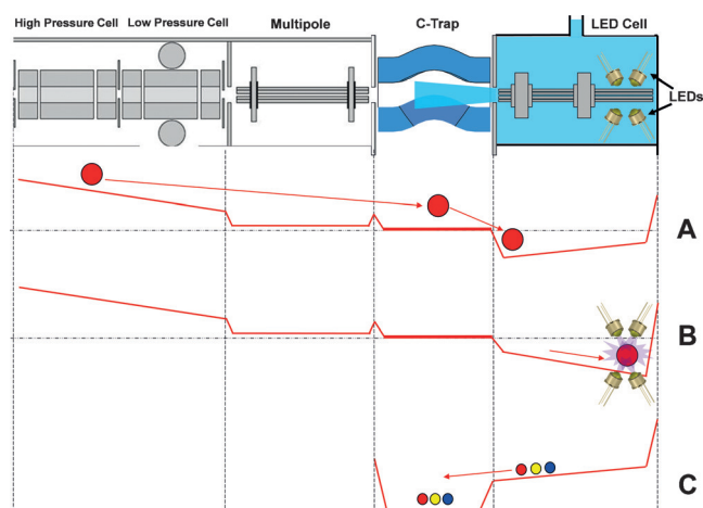
Figure 3. LED-HCD cell with overlays of applied potentials during various experimental steps: A) Ions are transferred to the front of the cell, B) ions are moved to the back of the cell and irradiated, and C) ions are transferred to the C-trap.
